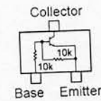
DTC114EK (24) (Q9501)
