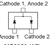
MC2850 (A7) (D1015, 1033, 1034, 1036)
