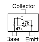
RT1P441U (P3) (Q1013, 1020, 1059)
