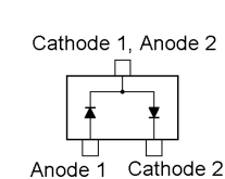
MC2850 (A7) (D1030)
