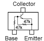
RT1N441U (N3) (Q1034, 1045, 1063)
