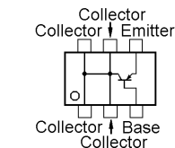
Collector Collector Emitter Collector Base Collector CPH6102 (AB) (Q1029, 1031)
