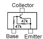
RT1P441U (P3) (Q1013, 1020, 1059)
