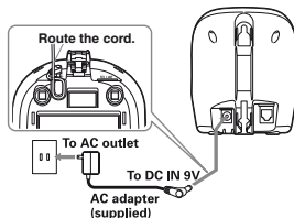
AC adapter
