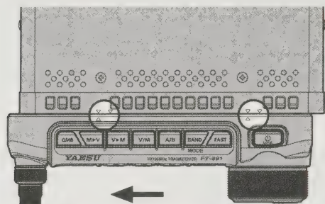
Slide the Front Panel
